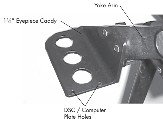
Typical DSC / Computer mounting plate on right Caddy. Note focuser knob clearance with plate (arrow).
